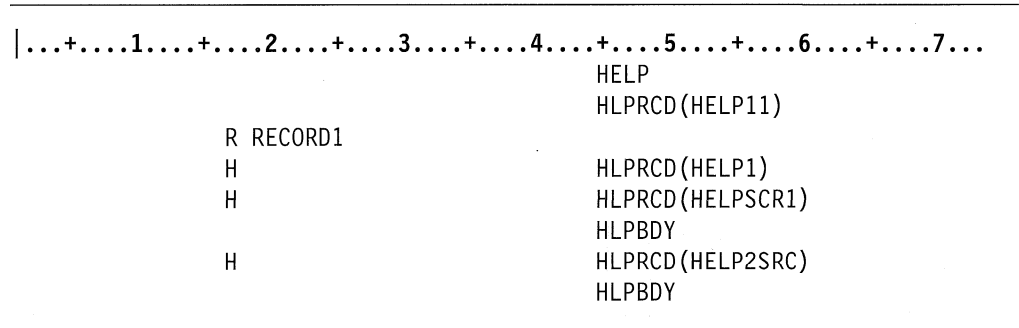
Figure 18-9. Sample DDS Source to Show Secondary Help
