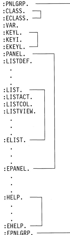
Figure 16-5. Required UIM Tags for a List Panel
