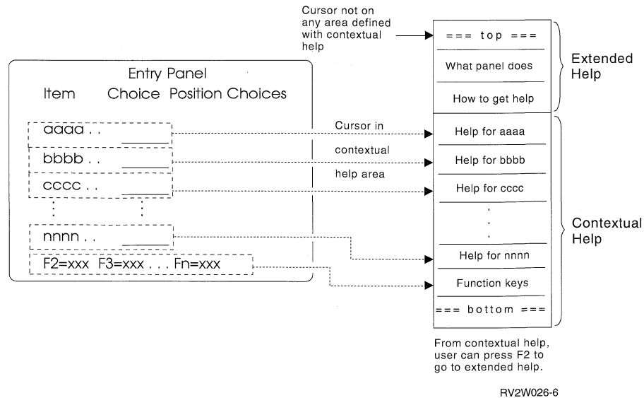
Figure 21-14. Help Areas for Entry Displays
