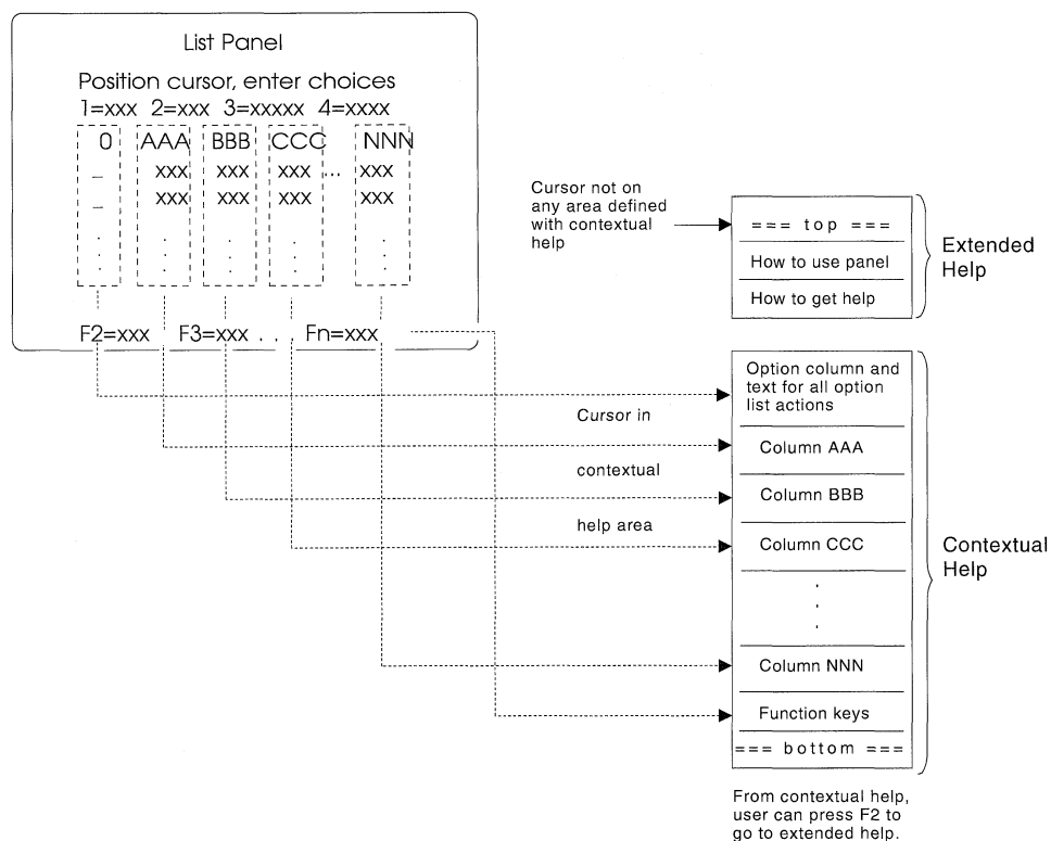
Figure 21-16. Help Areas for List Displays
