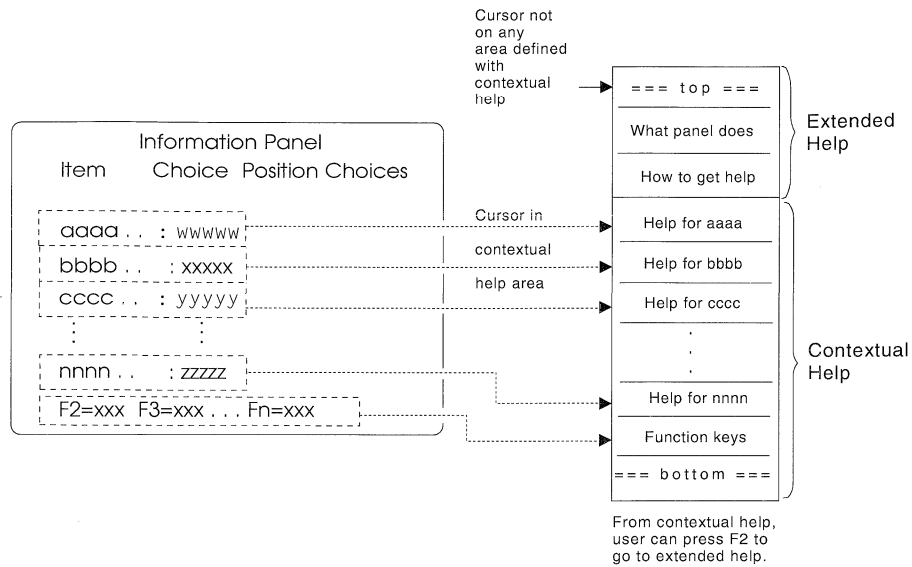
Figure 21-15. Help Areas for Information Displays
